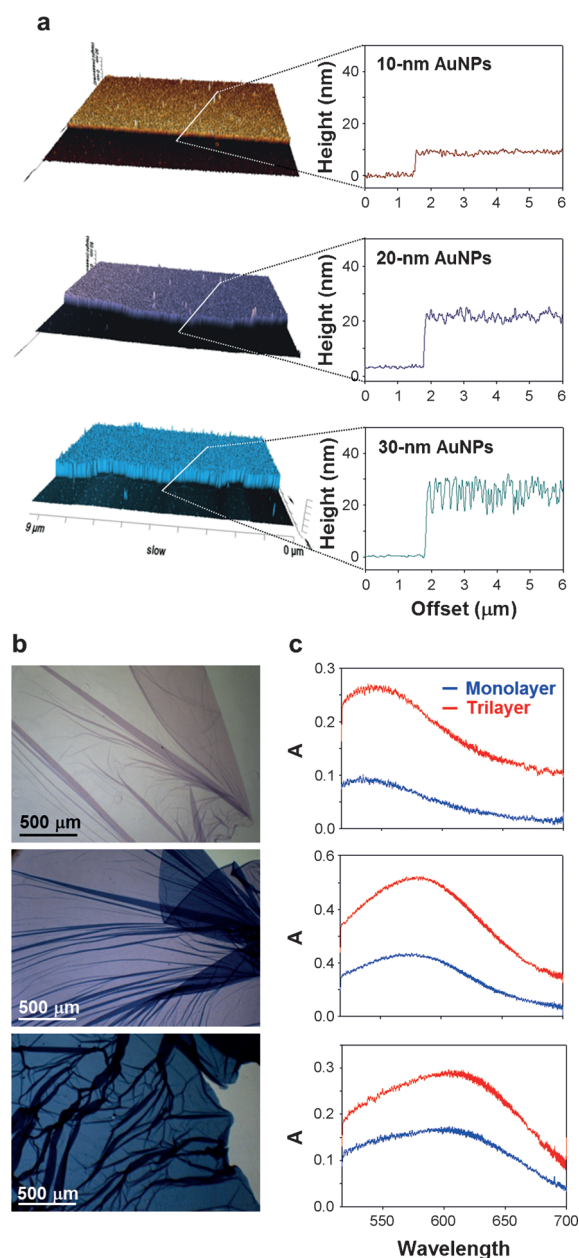
Figure 3. \alpha S-AuNP monolayer films produced with 10 nm diameter AuNPs (top row), 20 nm diameter AuNPs (middle row), and 30 nm diameter AuNPs (bottom row). a) Three-dimensional AFM images of the \alpha S-AuNP films showing the thickness profiles. b) Optical microscope images of the \alpha S-AuNP films. c) SPR spectra of the films acquired by monitoring local absorbance of the films with a Reinshaw InVia Raman spectrometer. The red and blue curves indicate the adsorption spectra of the \alpha S-AuNP films in triple layers and single layers, respectively.
